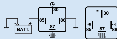
POSITION OF FLAT TERMINALS TO ISO 7588
